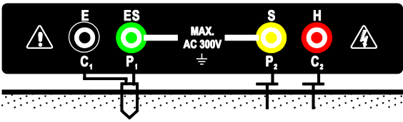
(1) Earth electrode (rod) under test (2) Potential spike (3) Current spike
